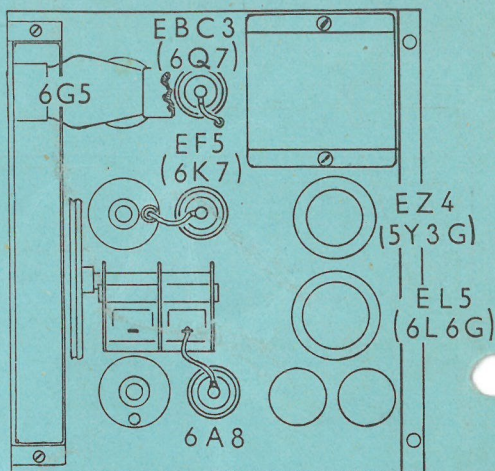
Chassis (overside)
